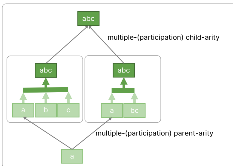
Figure 16: Participation (as composite or component) relation
